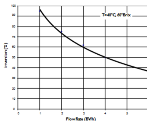
Figure 4: Inversion vs. Flowrate
